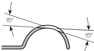
Figure 2: Maintain these angles when you sharpen.
