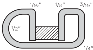
Figure 1: Use to sharpen inside radius of tools.
